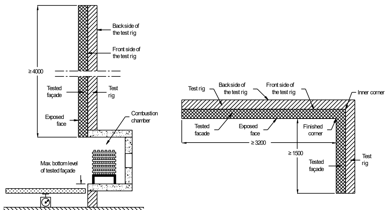
Figure 6. Test specimen and test rig (minimal dimensions).
