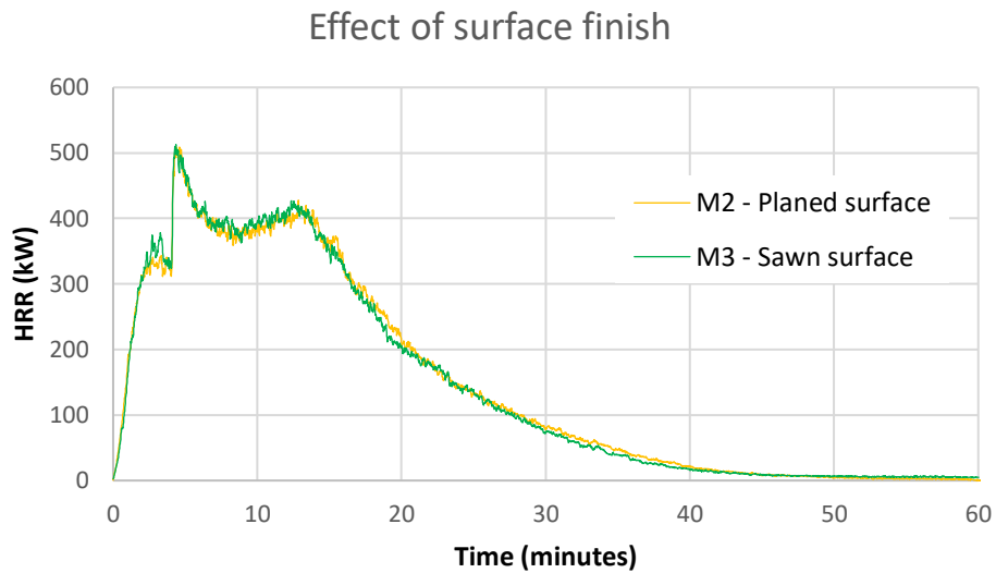
Figure F17. Heat release rate obtained with cribs M2 and M3.
