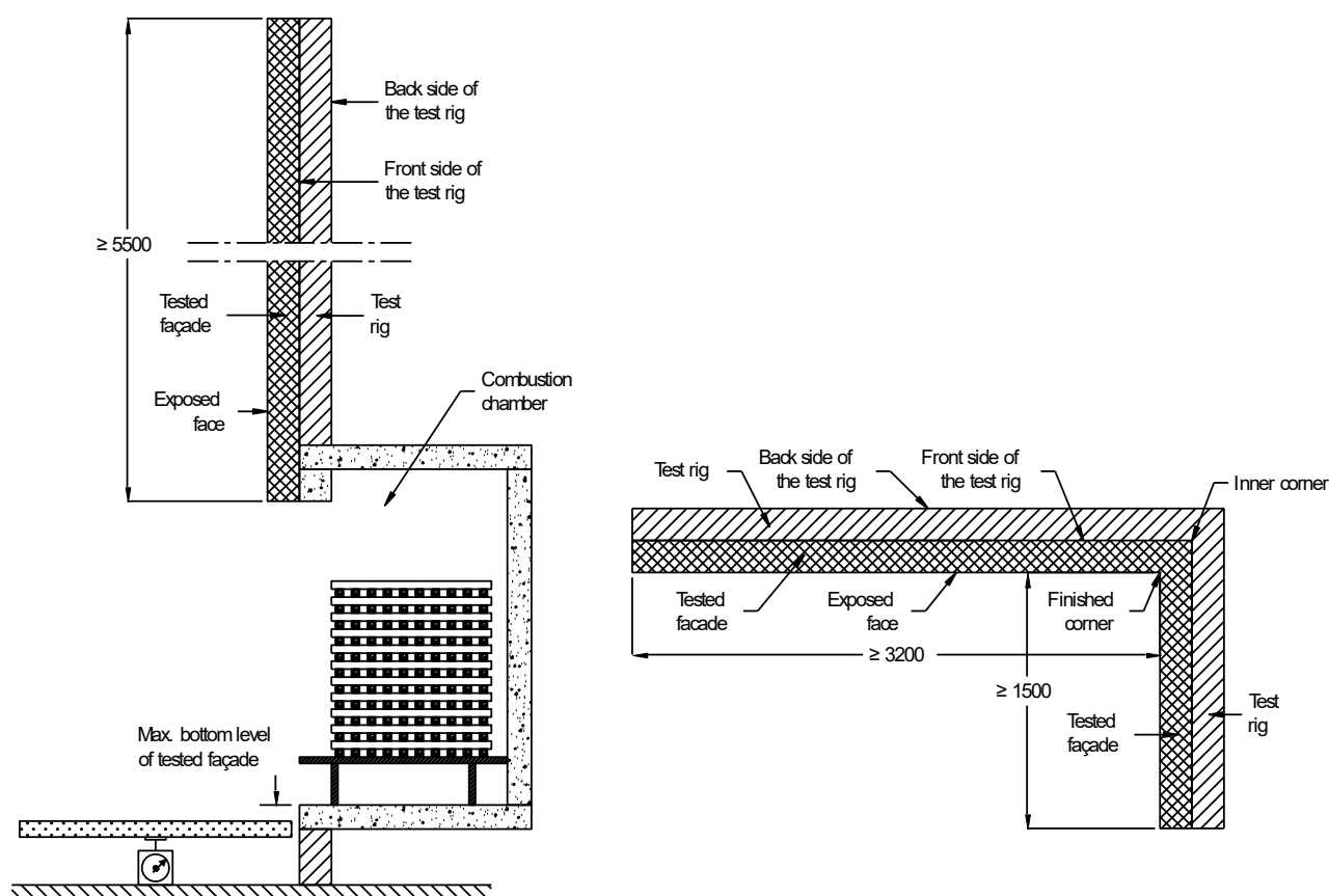
Figure 7. Test specimen and test rig (minimal dimensions).
