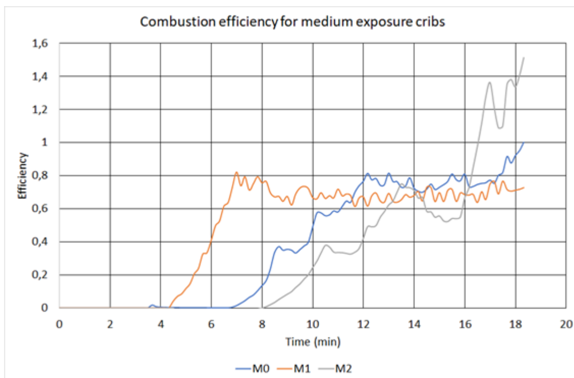
Figure F5. Comparison of efficiencies for medium exposure cribs
