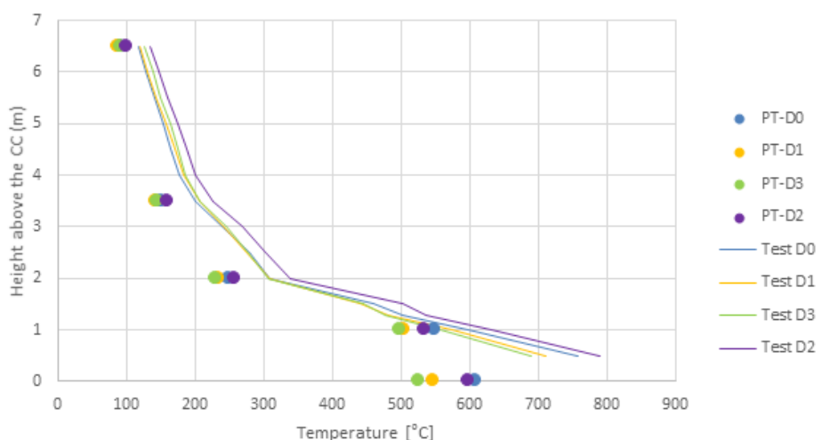
Figure H2. Temperature distribution on the central axis above the combustion chamber (CC) for test series D (repeatability, 400 m³/h air into the CC). Lines and symbols represent TC- and PT measurements, respectively.
