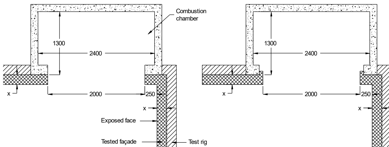
Figure 8c. Horizontal section of the detailing at the edges of openings schematically exemplified. The general closing configuration is shown on the left, the detail as in practice is shown on the right, x refers to the actual thickness of the tested façade.
