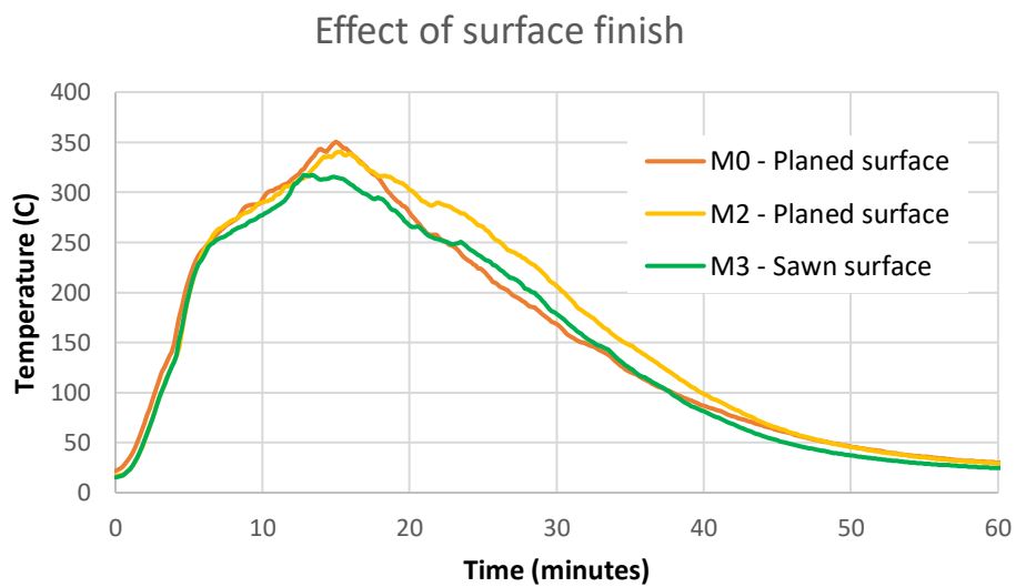
Figure F18. Temperatures measured with plate thermometer 1 m above the upper edge of the combustion chamber with cribs M0, M2 and M3.
