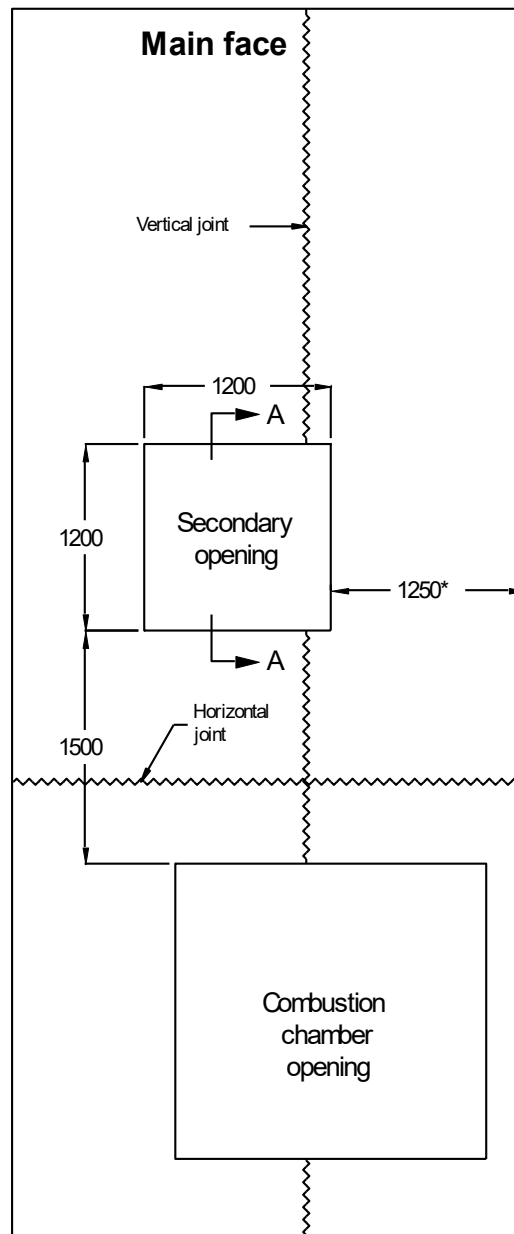
Figure 6.1 Main face with secondary opening including the location of vertical and horizontal joints. Distances in the drawing have to be considered with a tolerance of \pm 50 mm except the vertical distance between corner and secondary opening which is 1250 \pm 100 mm.
