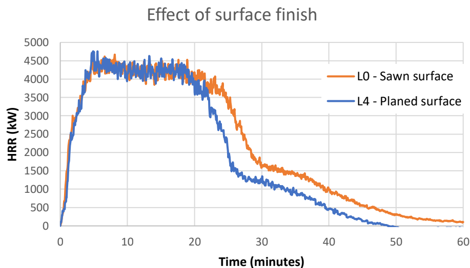
Figure F19. Heat release rate obtained with pine cribs L0 ( \rho=490 \text{ kg/m}^3 , MC=11.5 \% ) and L4 ( \rho=485 \text{ kg/m}^3 , MC=11.7 \% ).
