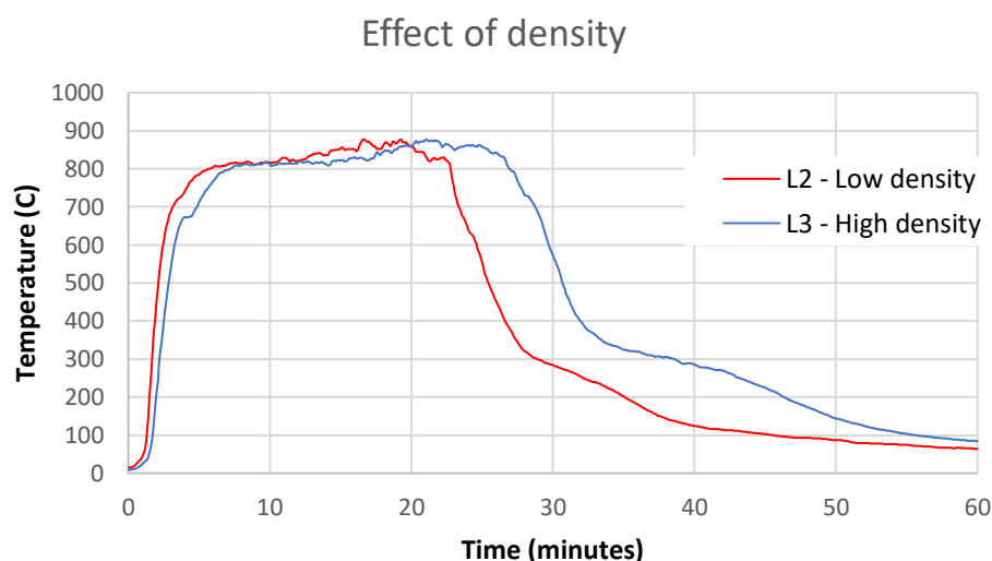
Figure F16. Temperature measured with plate thermometer 1 m above the upper edge of the combustion chamber. The average densities of L2 and L3 were 301 and 400 kg/m 3 , respectively.
